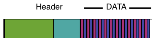
1/4 msec packet (WNIP) 12 Stereo audio samples, L-R Interleaved
